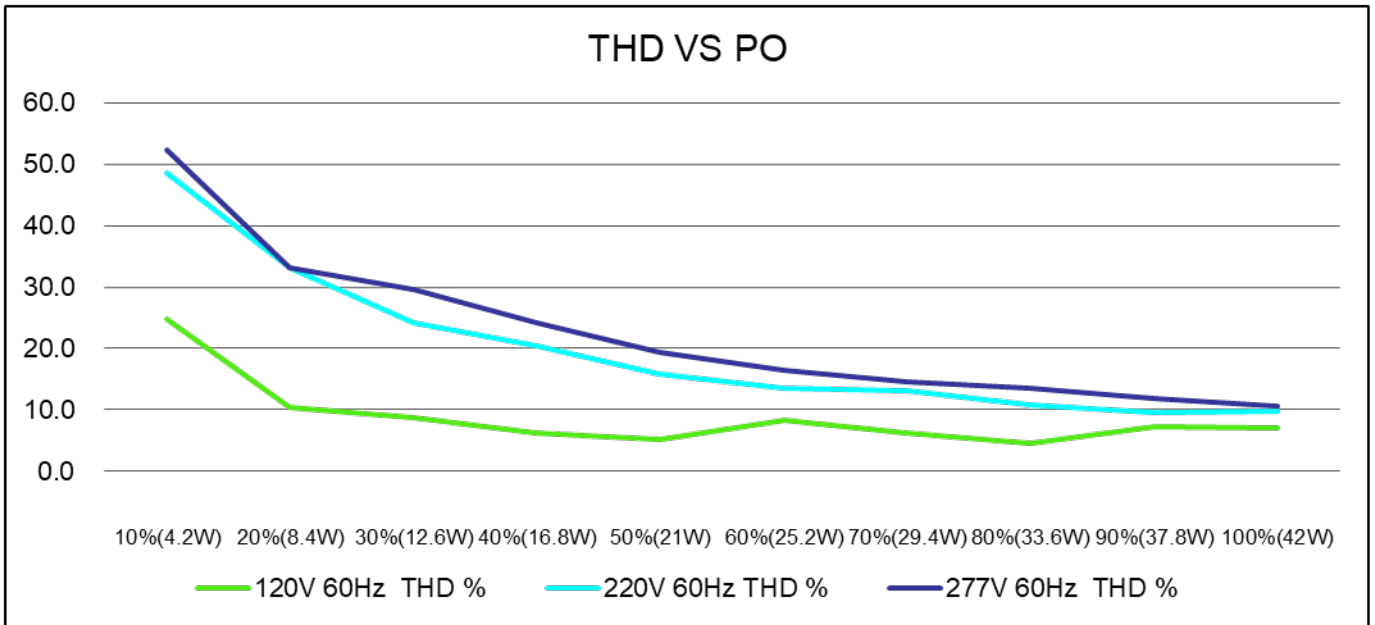
THD of the driver VS Power Output (W) :
